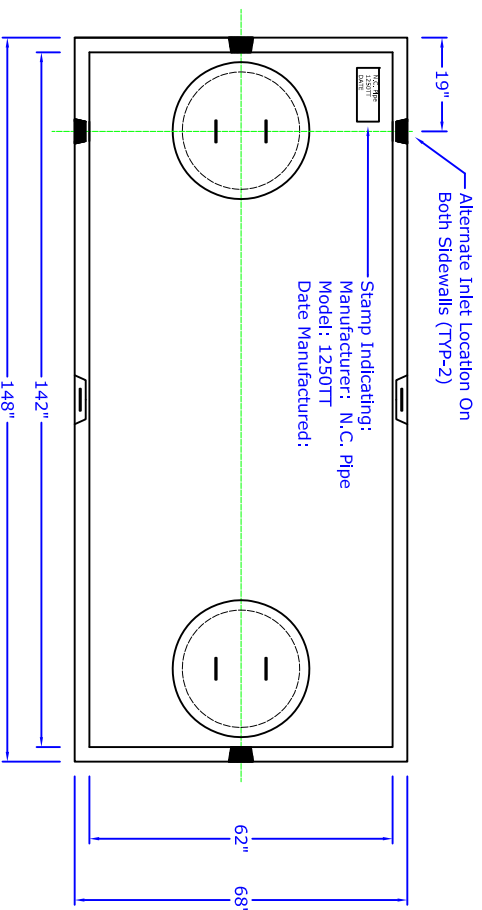
PLAN VIEW
