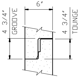
60" JOINT DETAIL
