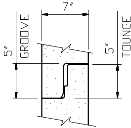
72" JOINT DETAIL
