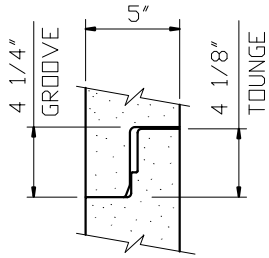
48" JOINT DETAIL
