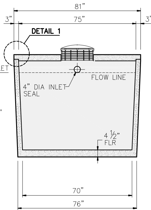
SECTION B-B
