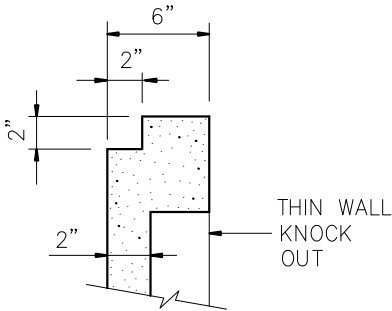
TYP. WALL DETAIL 48" X 48"
