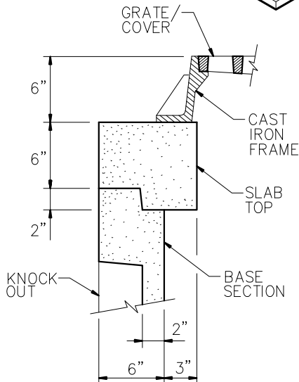
TYPICAL WALL SECTION
