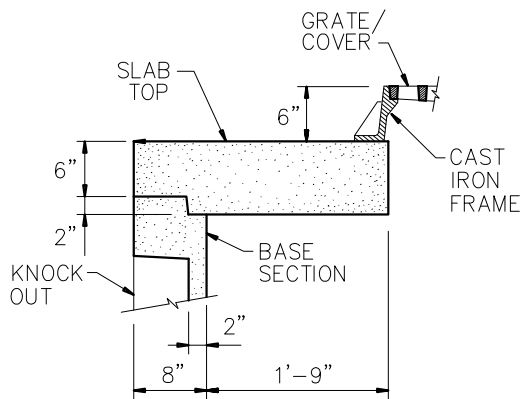
TYPICAL WALL SECTION
